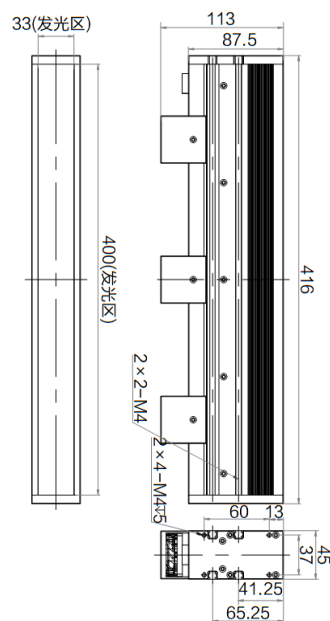
MV-LTHS-400-WX
