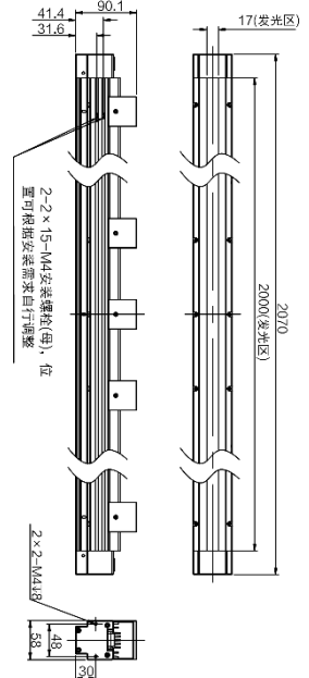
MV-LTHS-2000-W
