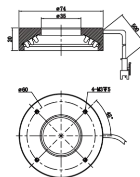
MV-LRM-74-60-W/IR940
