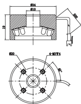
MV-LRM-34-75-W/B
