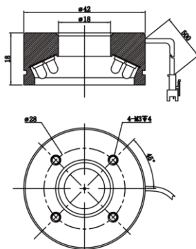
MV-LRM-42-65-W
