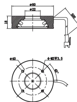
MV-LRM-60-30-W/B
