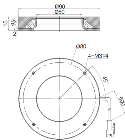
MV-LRM-90-45
