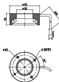
MV-LRM-52-60-W/IR940/B
