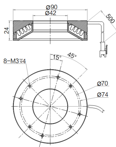
MV-LRM-90-60-W
