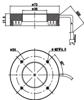
MV-LRM-73-90-W/IR940
