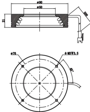
MV-LRM-90-30-W/IR940
