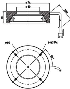
MV-LRM-74-30-W/IR940
