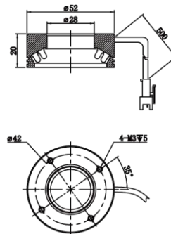
MV-LRM-52-60-W/IR940/B
