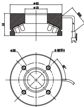
MV-LRM-42-65-W
