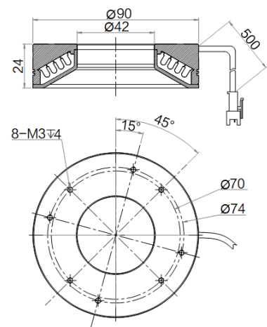
MV-LRM-90-60-W
