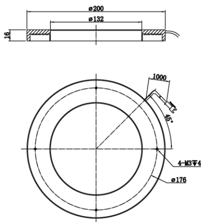
MV-LRM-200-90-W
