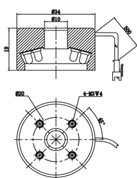
MV-LRM-34-75-W/B
