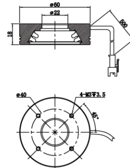
MV-LRM-60-30-W/B
