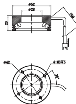
MV-LO-52-60-W/IR940/B
