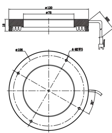
MV-LO-120-90-W
