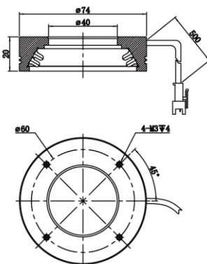
MV-LO-74-30-W/IR940
