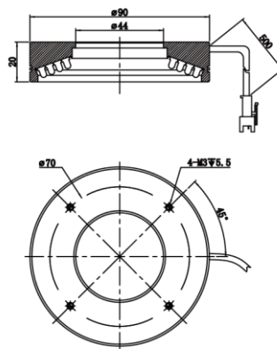
MV-LO-90-70-W/R
