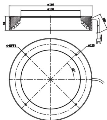
MV-LO-140-45-W
