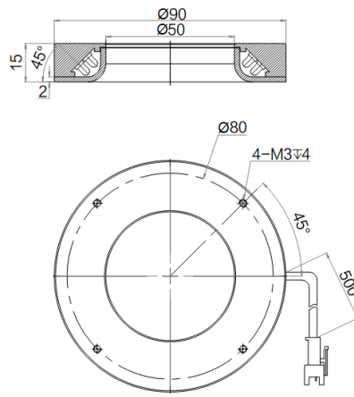
MV-LO-90-45
