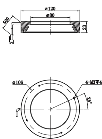
MV-LO-120-30-W/B
