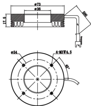
MV-LO-73-90-W/IR940
