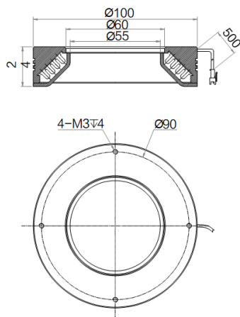
MV-LO-100-45-W
