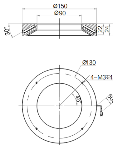
MV-LO-150-60-W
