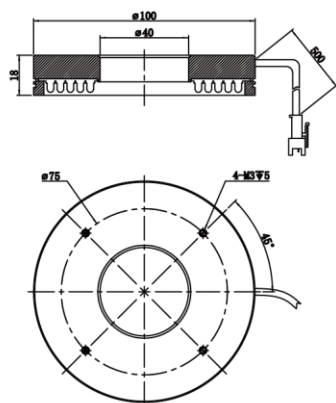
MV-LO-100-90-W/R
