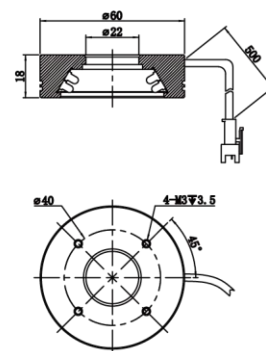
MV-LO-60-30-W/B
