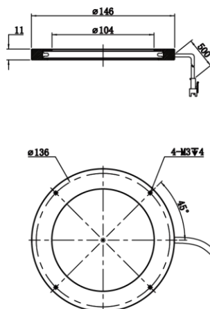
MV-LO-146-0-W/IR940
