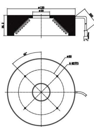
MV-LO-120-45-W
