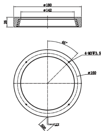
MV-LO-180-15-W
