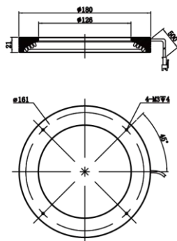
MV-LO-180-60-W
