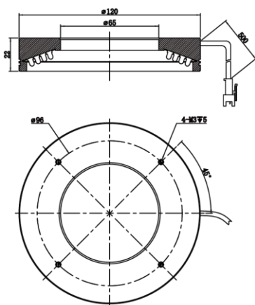
MV-LO-120-70-W
