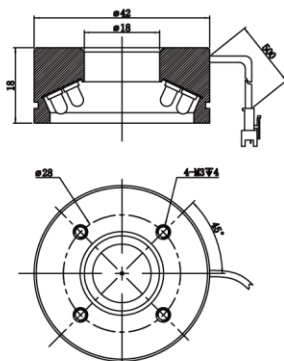
MV-LO-42-65-W
