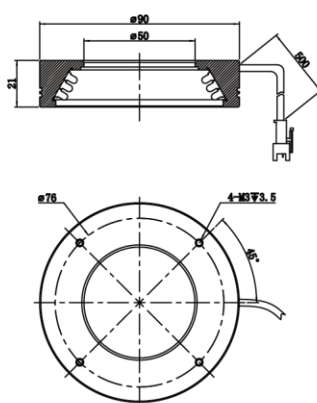
MV-LO-90-30-W/IR940
