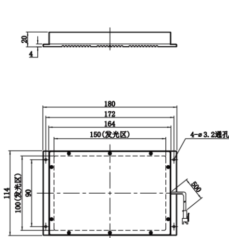
MV-LBSS-150-100-W
