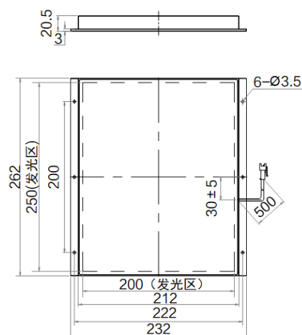
MV-LBSS-250-200-W
