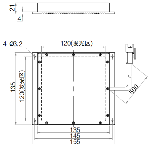
MV-LBSS-120-120-W/R
