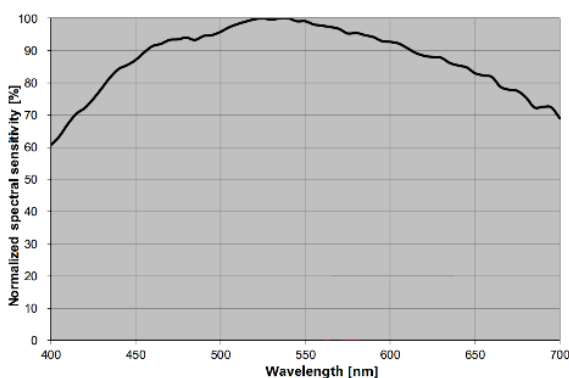
MV-CH1510-10(11)XM
